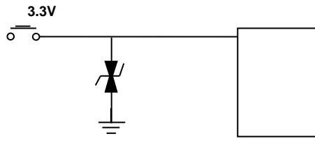
ESD3V3D3B
