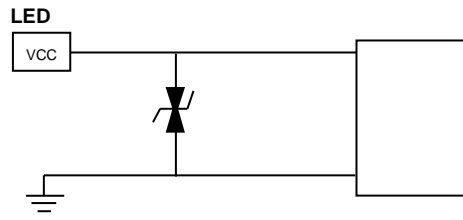
ESD3V3D3B
